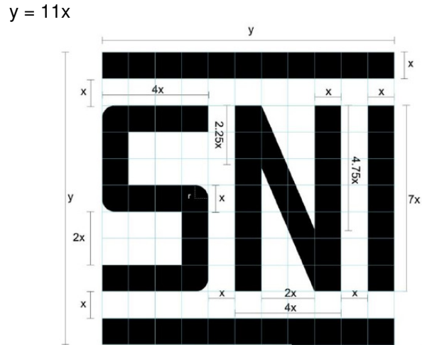
Figure 2. Size of SPPT SNI Marking
