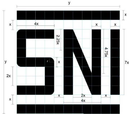
Figure 2. Size of SNI Marking
