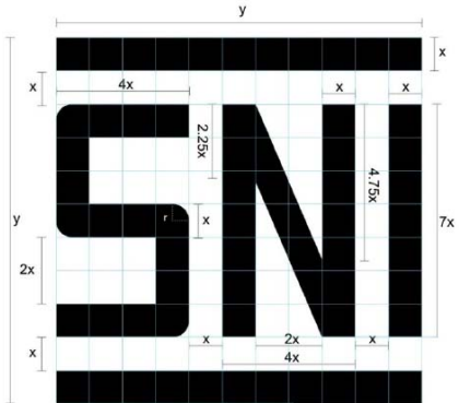
Gambar 2. Ukuran Tanda SNI
